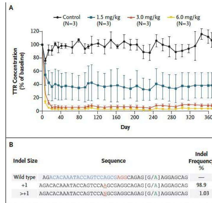
Figure 3. In Vivo Pharmacologic Properties of Cyn-LNP, the Nonhuman Primate Surrogate of NTLA-2001.
