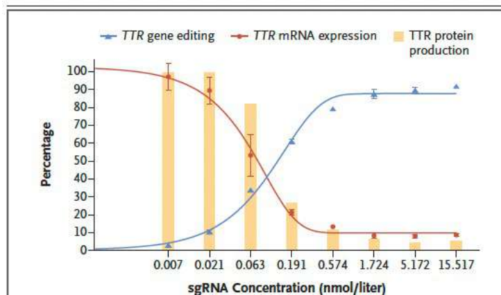
Figure 2. In Vitro Evaluations of the Potency of NTLA-2001.
